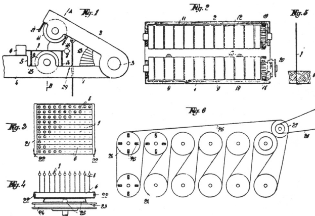
Figure 110. Machine for silvering beads with silver essence, Plessner method (Parkert 1925:175, Figure 40).
