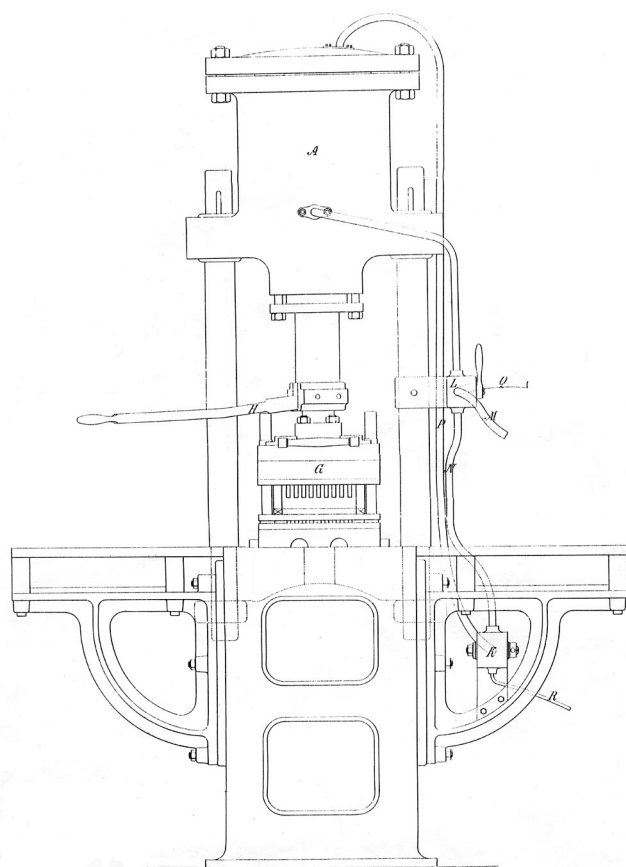
Figure 98. A hydraulic pressing system for manufacturing buttons, beads, and other similar objects made from ceramic materials, 1880, J.F. Bapterosses, privilege no. 30/953 (Austrian Patent Office, Vienna).
