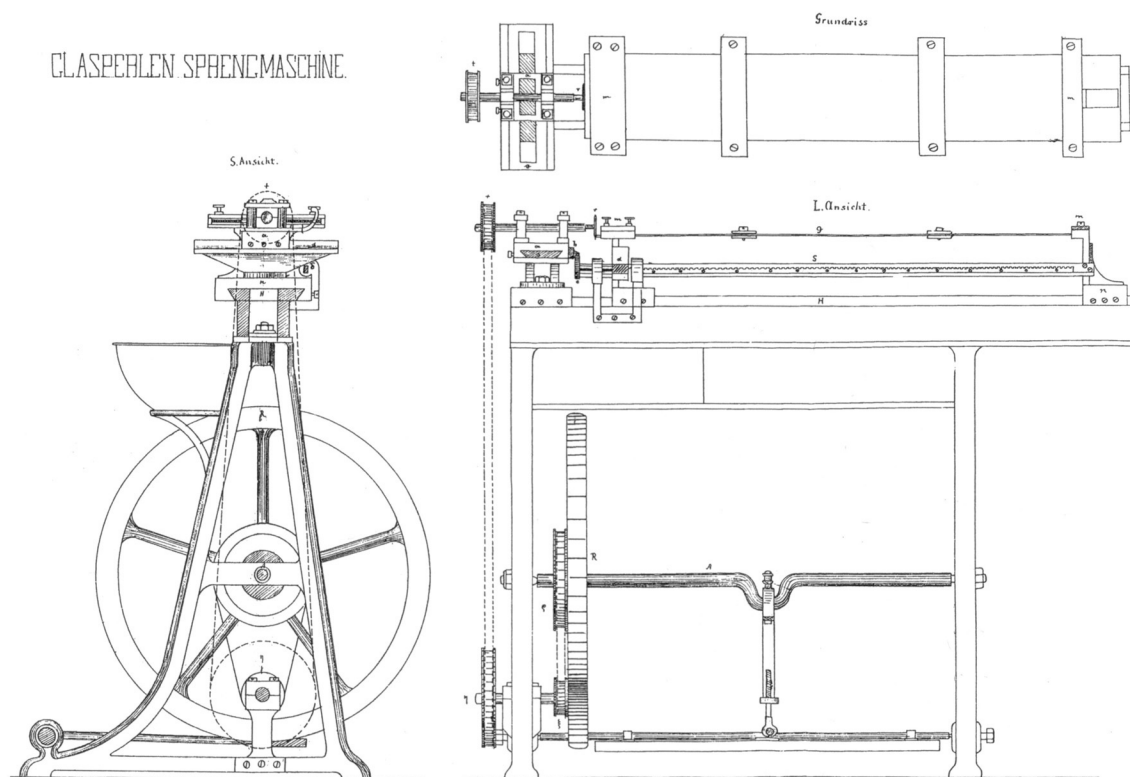
Figure 53. Machine for breaking off glass beads, 1877, Adolf Schindler, Vienna, privilege no. 27/112 (Austrian Patent Office, Vienna).
